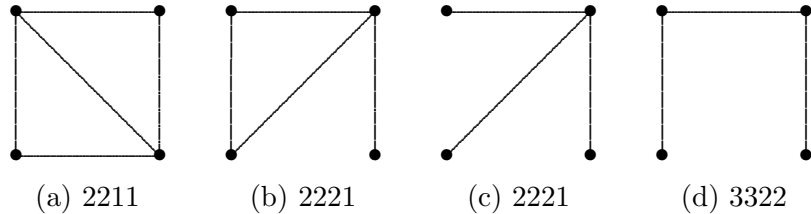
Figure 1: Some graphs and their eccentricity sequences
